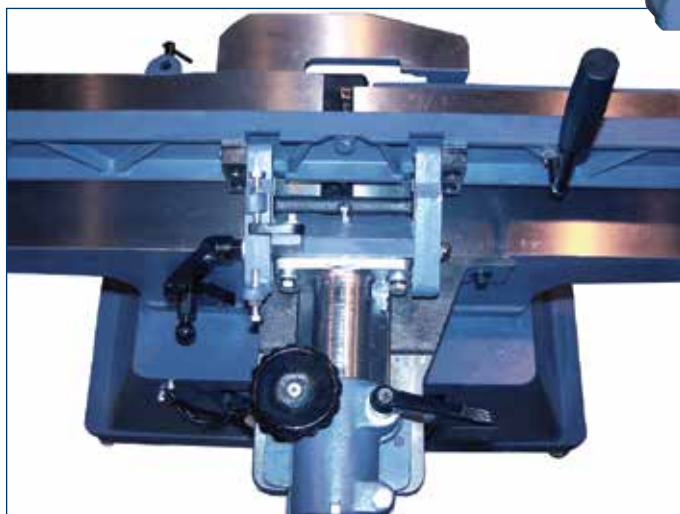
STANDARD helical cutterhead with GERMAN CARBIDE inserts is included with jointer.
